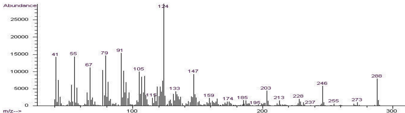
70 eV Electron Ionization Mass Spectrum
